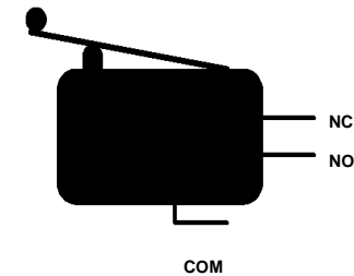
Rotation Microswitch Terminal Identification
