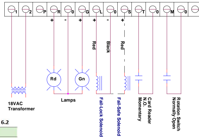
TCB 6.0, 6.1 & 6.2 Control Board (New Board)
